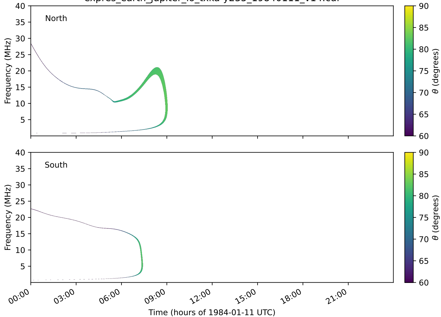
expres_earth_jupiter_io_txka-y235_19840111_v14.cdf
