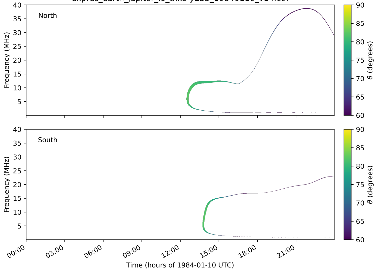
expres_earth_jupiter_io_txka-y235_19840110_v14.cdf
