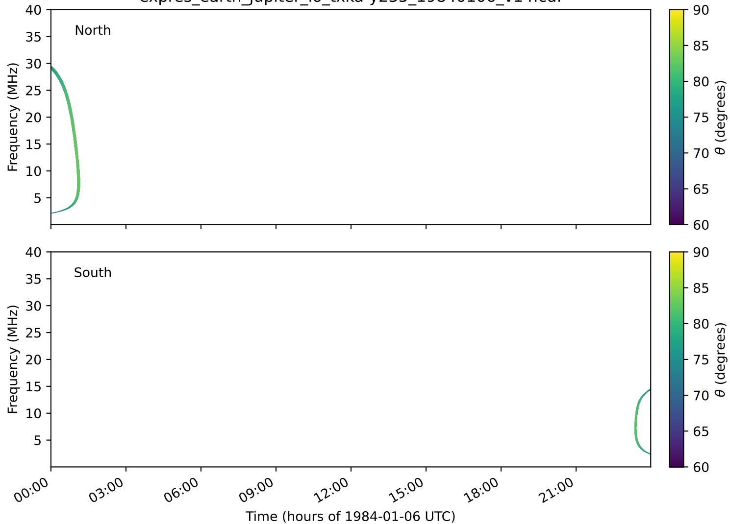
expres_earth_jupiter_io_txka-y235_19840106_v14.cdf
