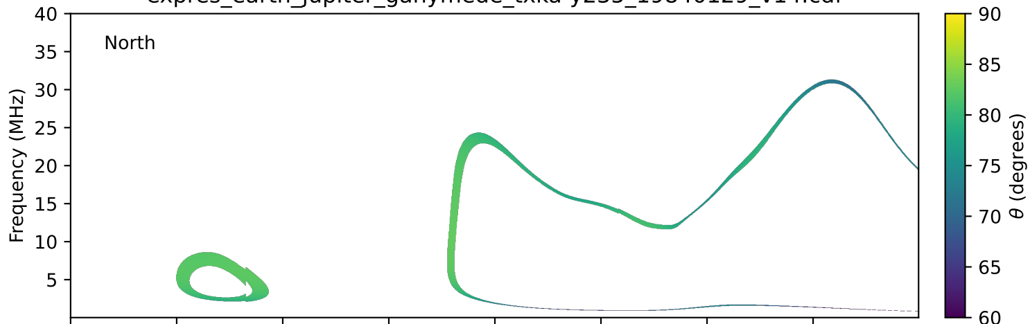
expres_earth_jupiter_ganymede_txka-y235_19840129_v14.cdf
