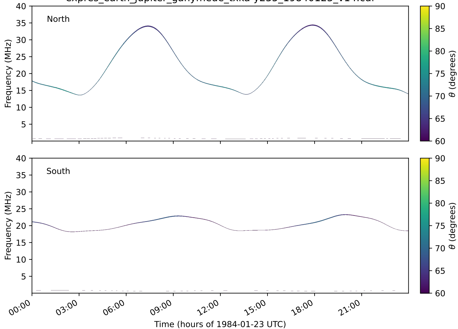
expres_earth_jupiter_ganymede_txka-y235_19840123_v14.cdf
