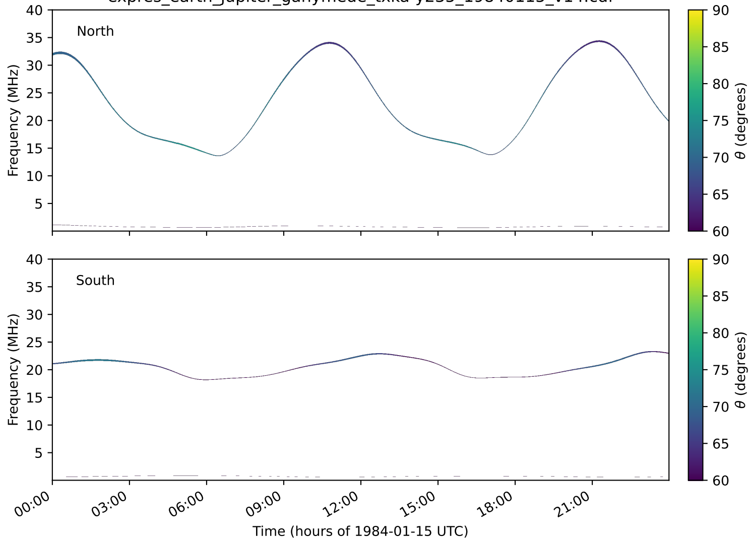
expres_earth_jupiter_ganymede_txka-y235_19840115_v14.cdf
