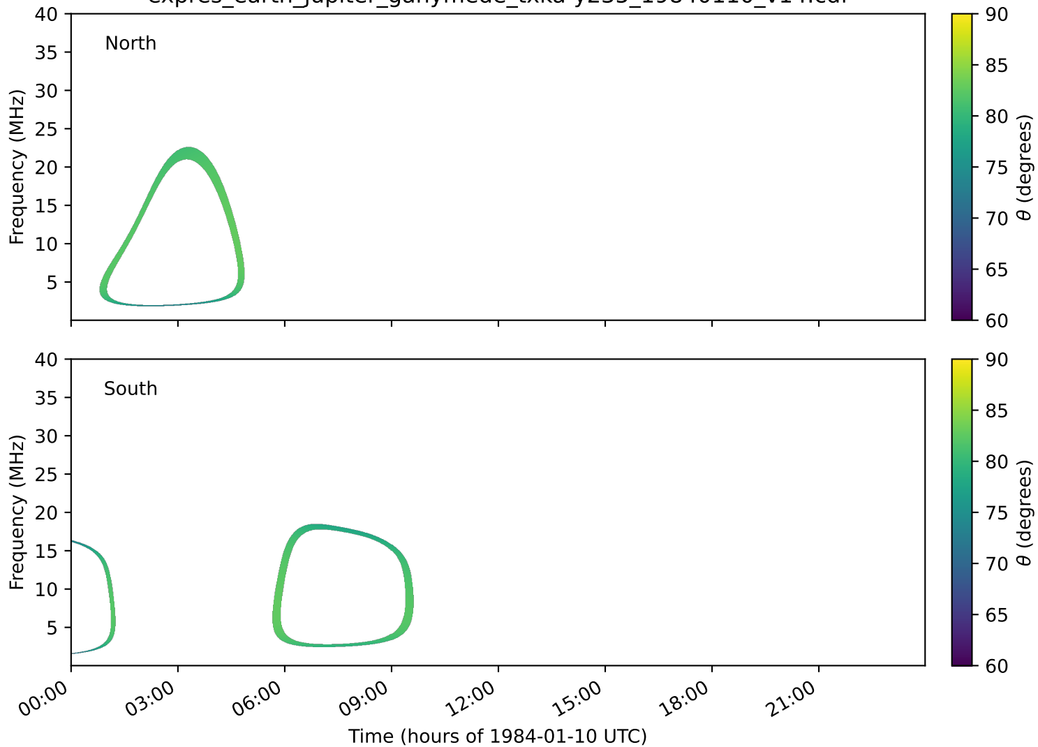
expres_earth_jupiter_ganymede_txka-y235_19840110_v14.cdf
