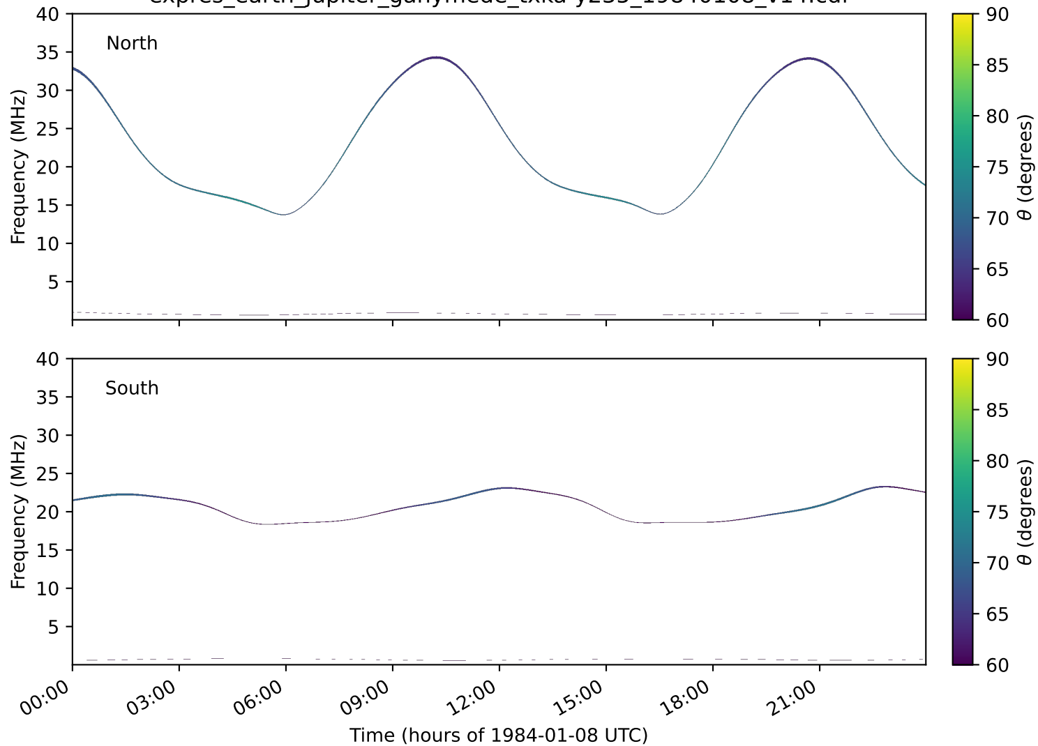
expres_earth_jupiter_ganymede_txka-y235_19840108_v14.cdf
