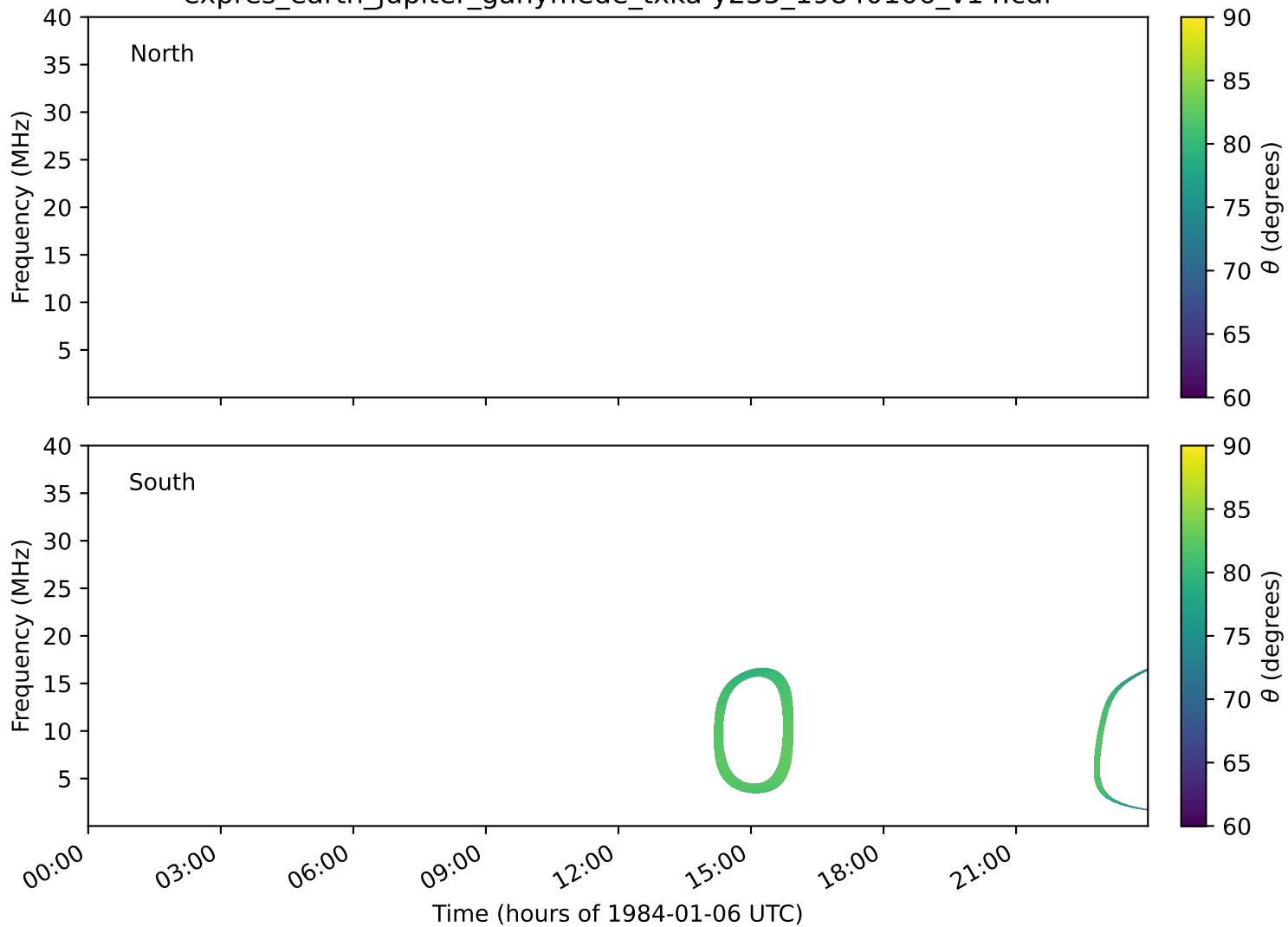
expres_earth_jupiter_ganymede_txka-y235_19840106_v14.cdf
