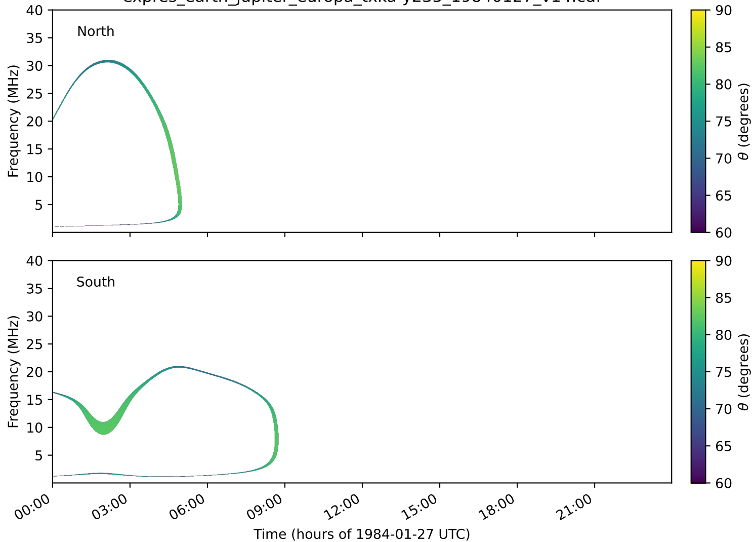
expres_earth_jupiter_europa_txka-y235_19840127_v14.cdf
