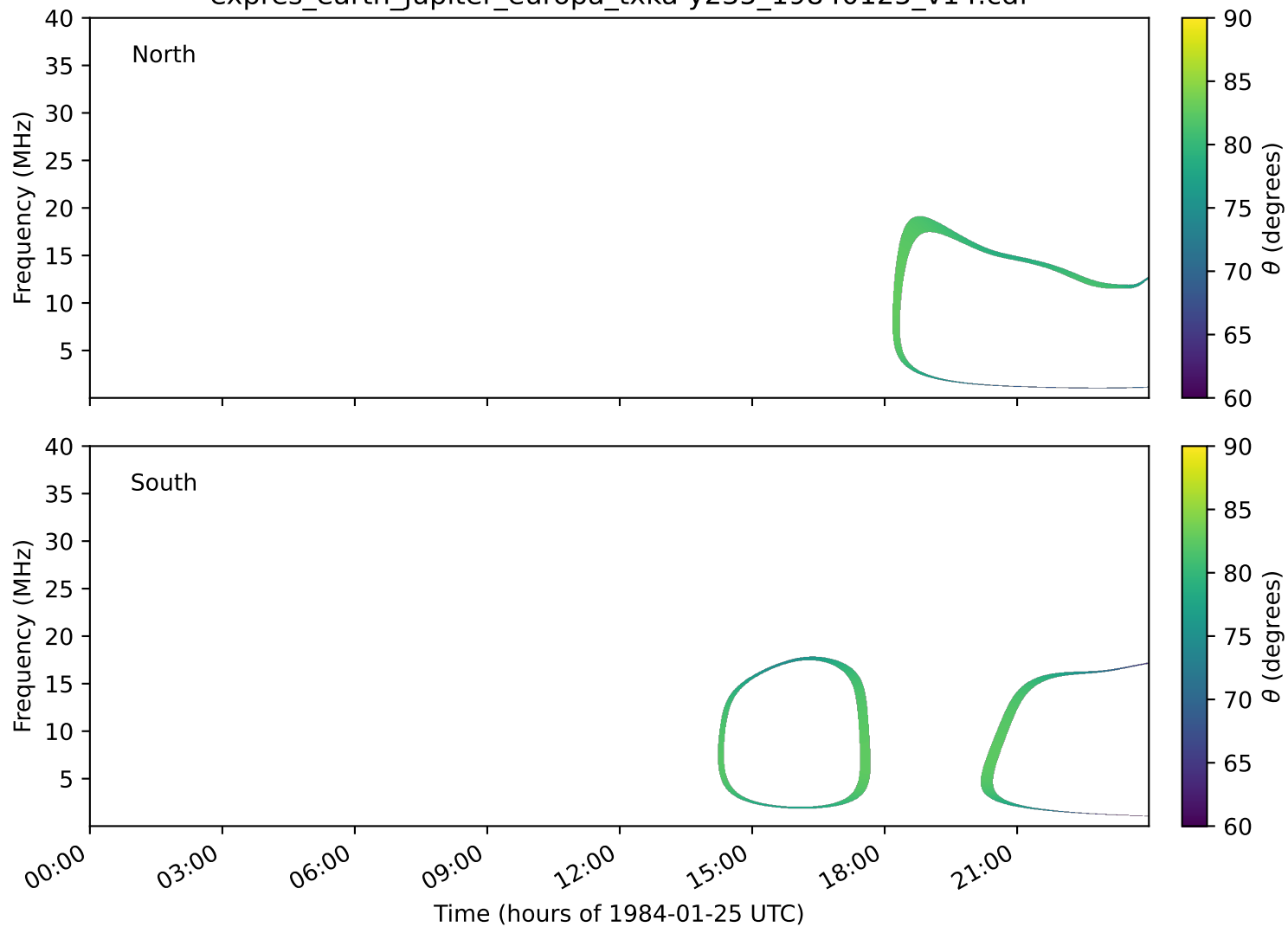
expres_earth_jupiter_europa_txka-y235_19840125_v14.cdf
