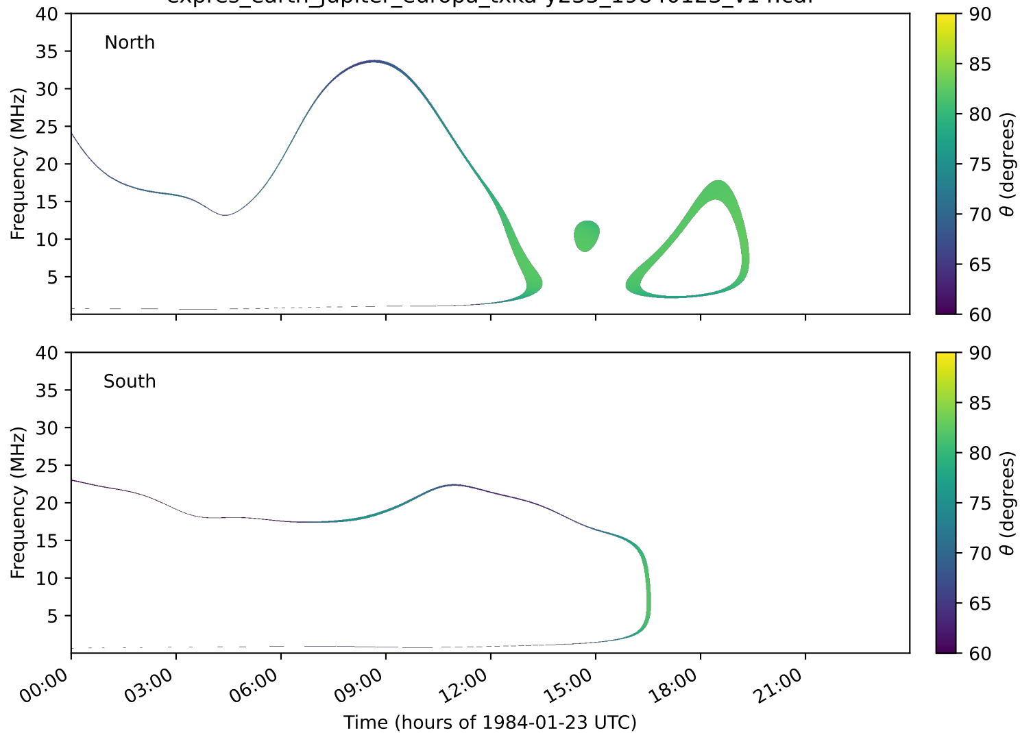
expres_earth_jupiter_europa_txka-y235_19840123_v14.cdf
