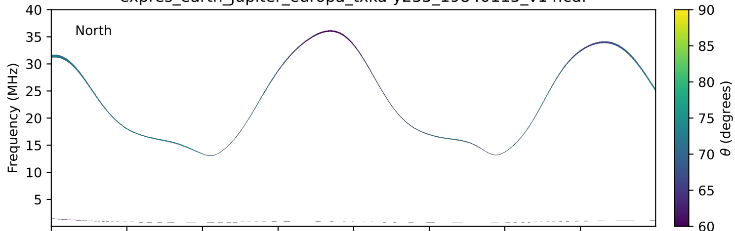
expres_earth_jupiter_europa_txka-y235_19840115_v14.cdf
