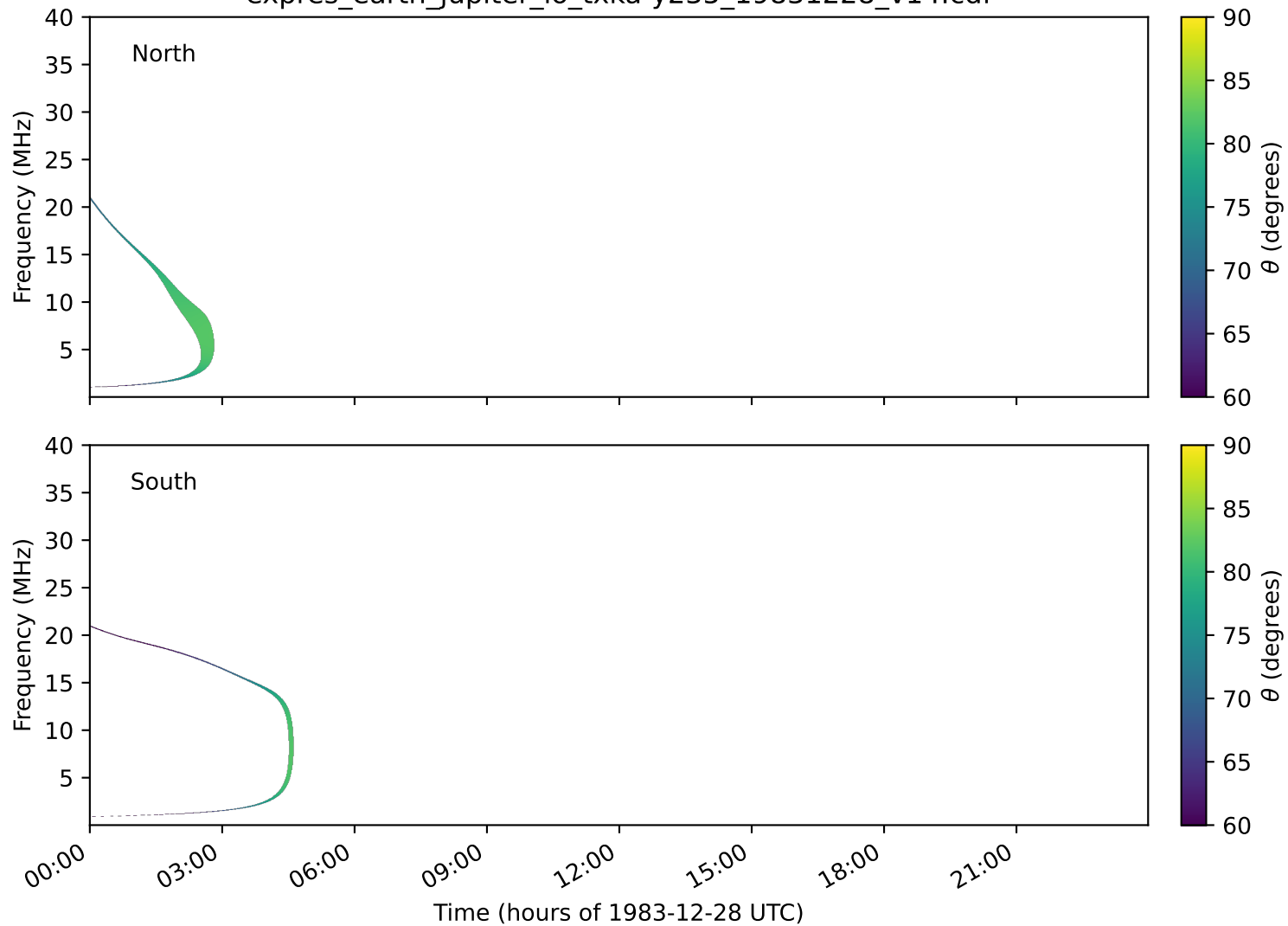
expres_earth_jupiter_io_txka-y235_19831228_v14.cdf
