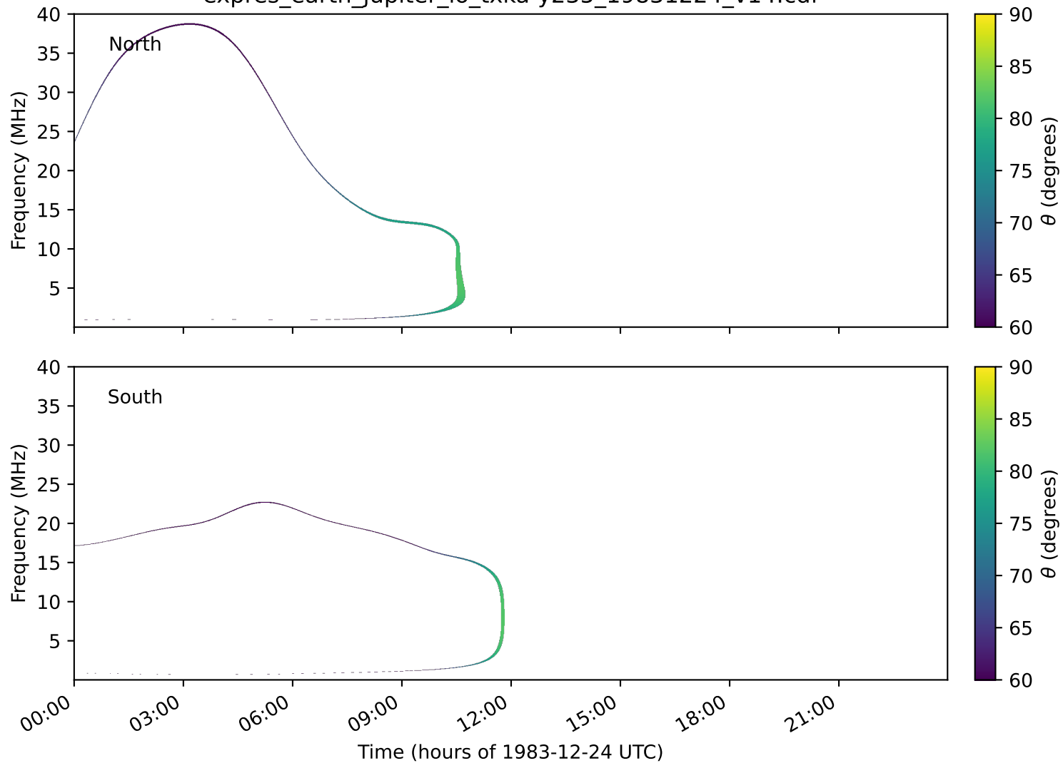
expres_earth_jupiter_io_txka-y235_19831224_v14.cdf
