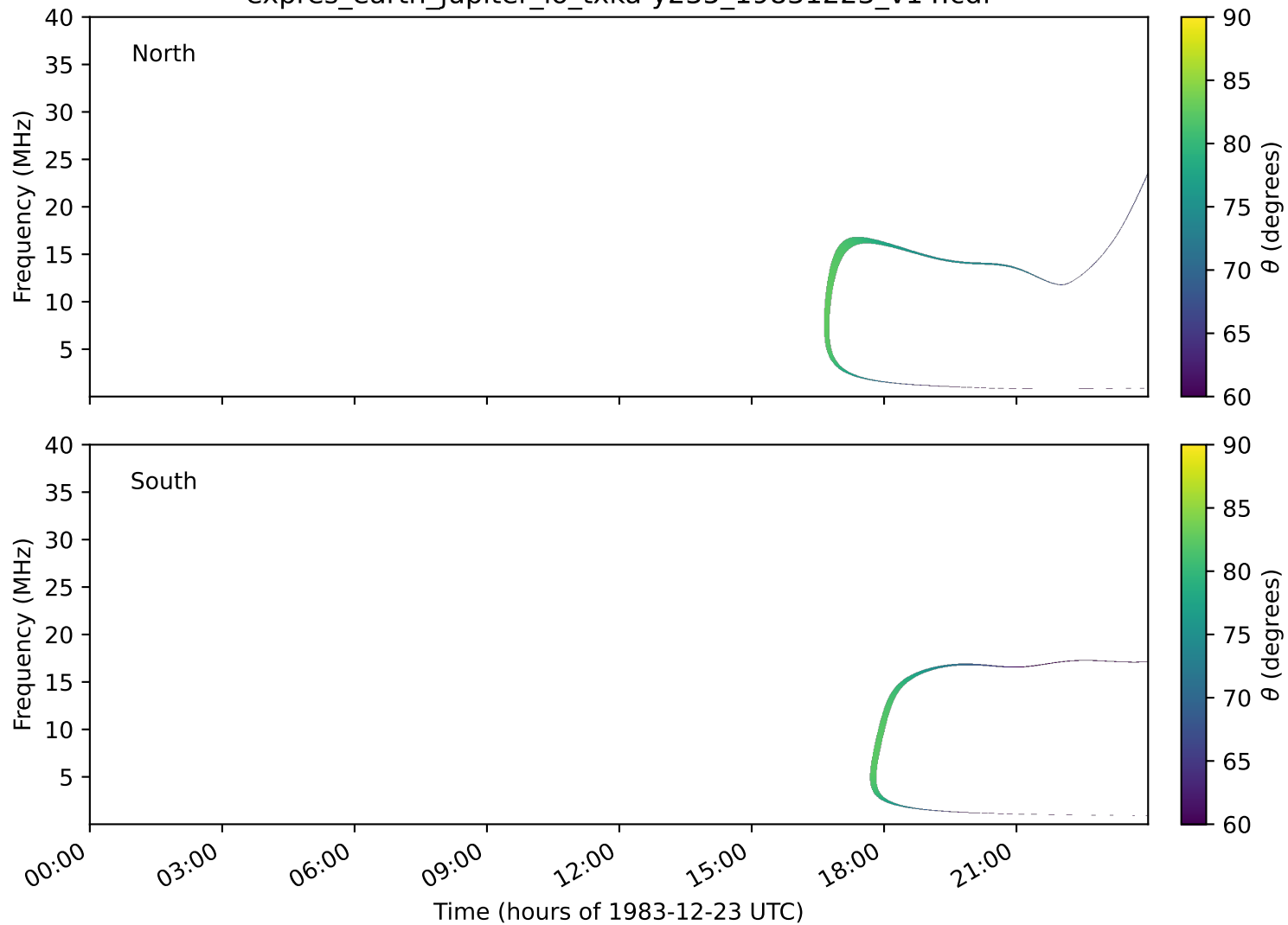
expres_earth_jupiter_io_txka-y235_19831223_v14.cdf
