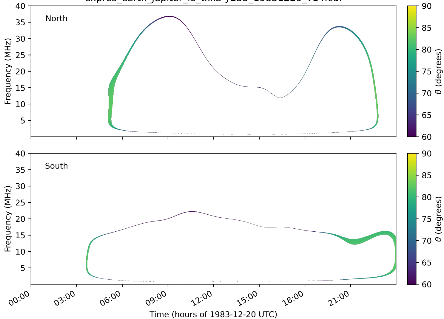
expres_earth_jupiter_io_txka-y235_19831220_v14.cdf
