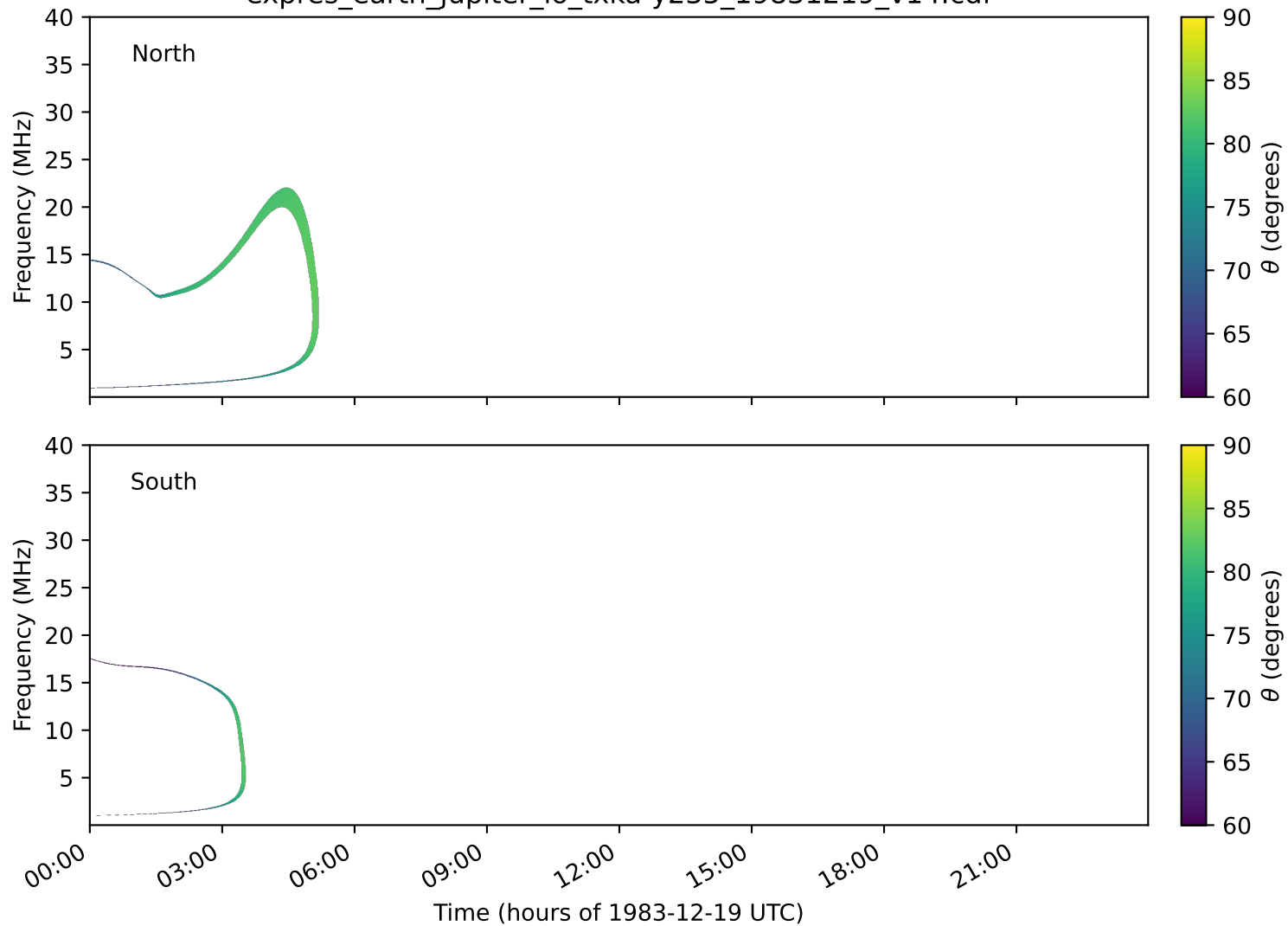
expres_earth_jupiter_io_txka-y235_19831219_v14.cdf
