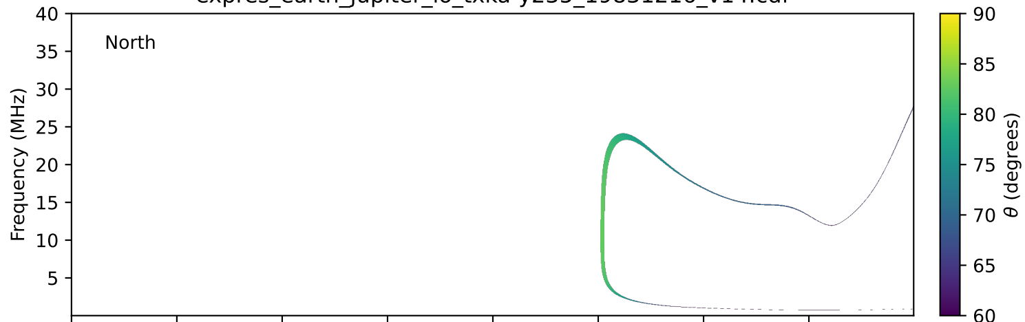
expres_earth_jupiter_io_txka-y235_19831216_v14.cdf
