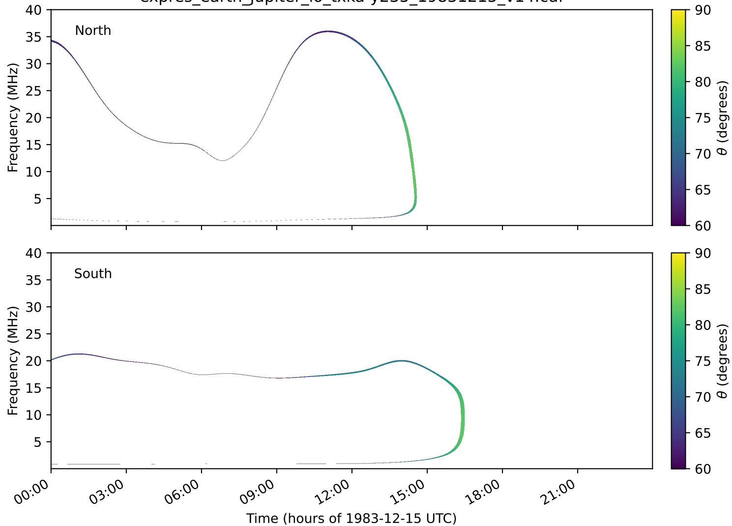
expres_earth_jupiter_io_txka-y235_19831215_v14.cdf
