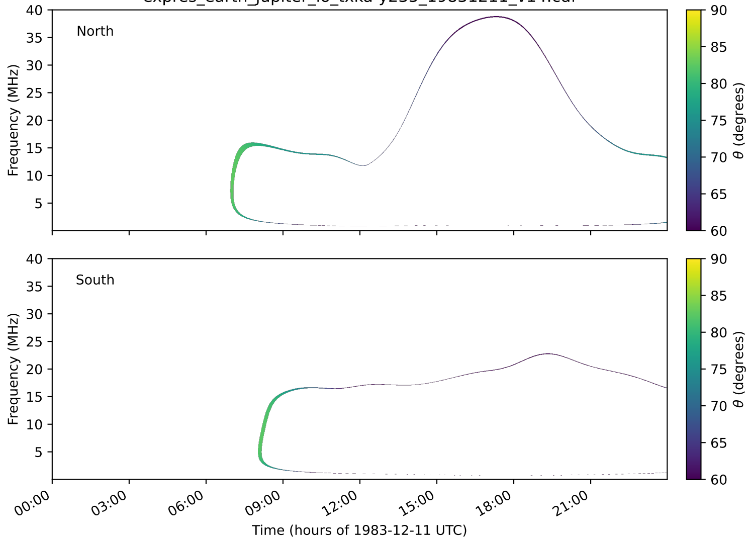
expres_earth_jupiter_io_txka-y235_19831211_v14.cdf
