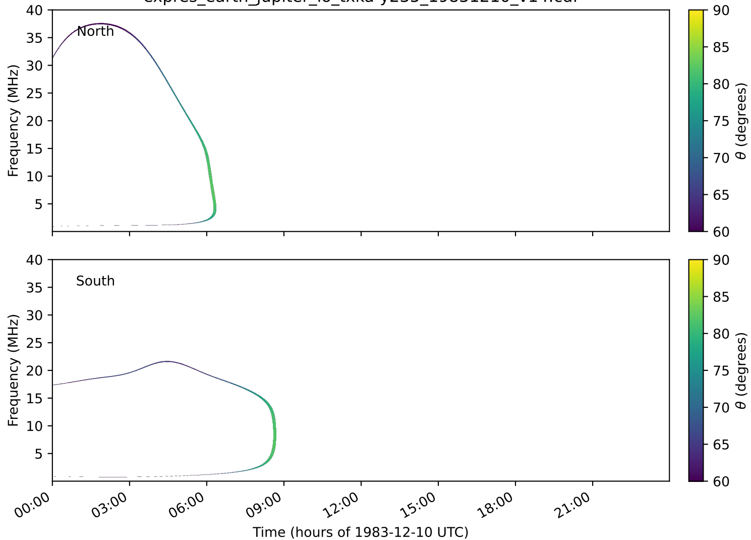
expres_earth_jupiter_io_txka-y235_19831210_v14.cdf
