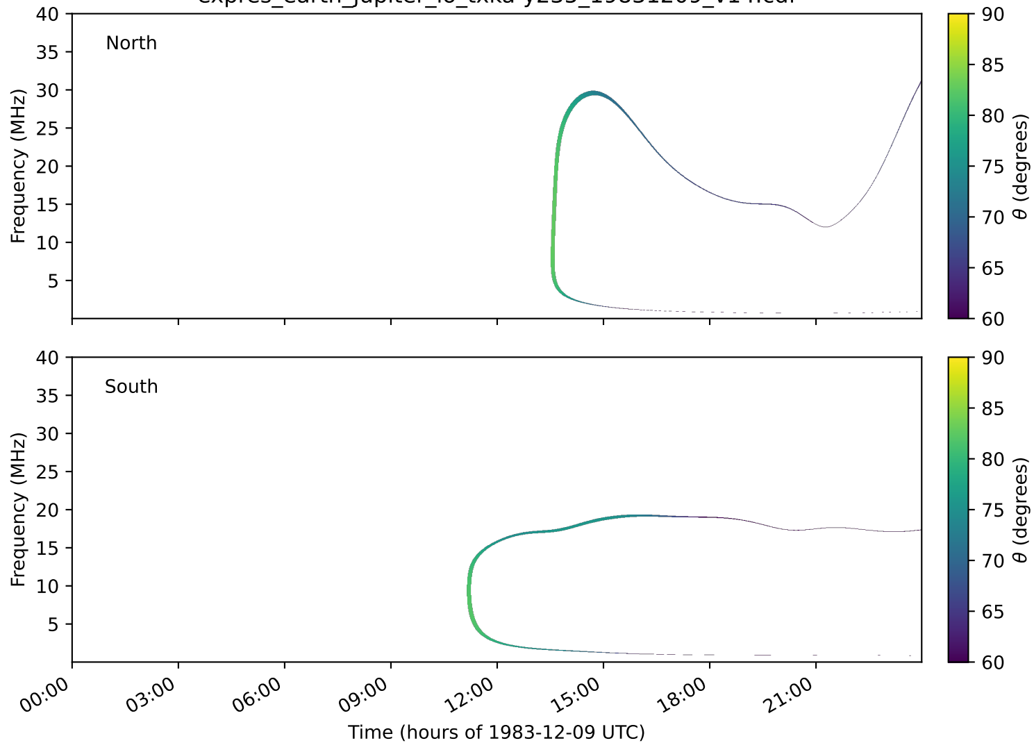
expres_earth_jupiter_io_txka-y235_19831209_v14.cdf
