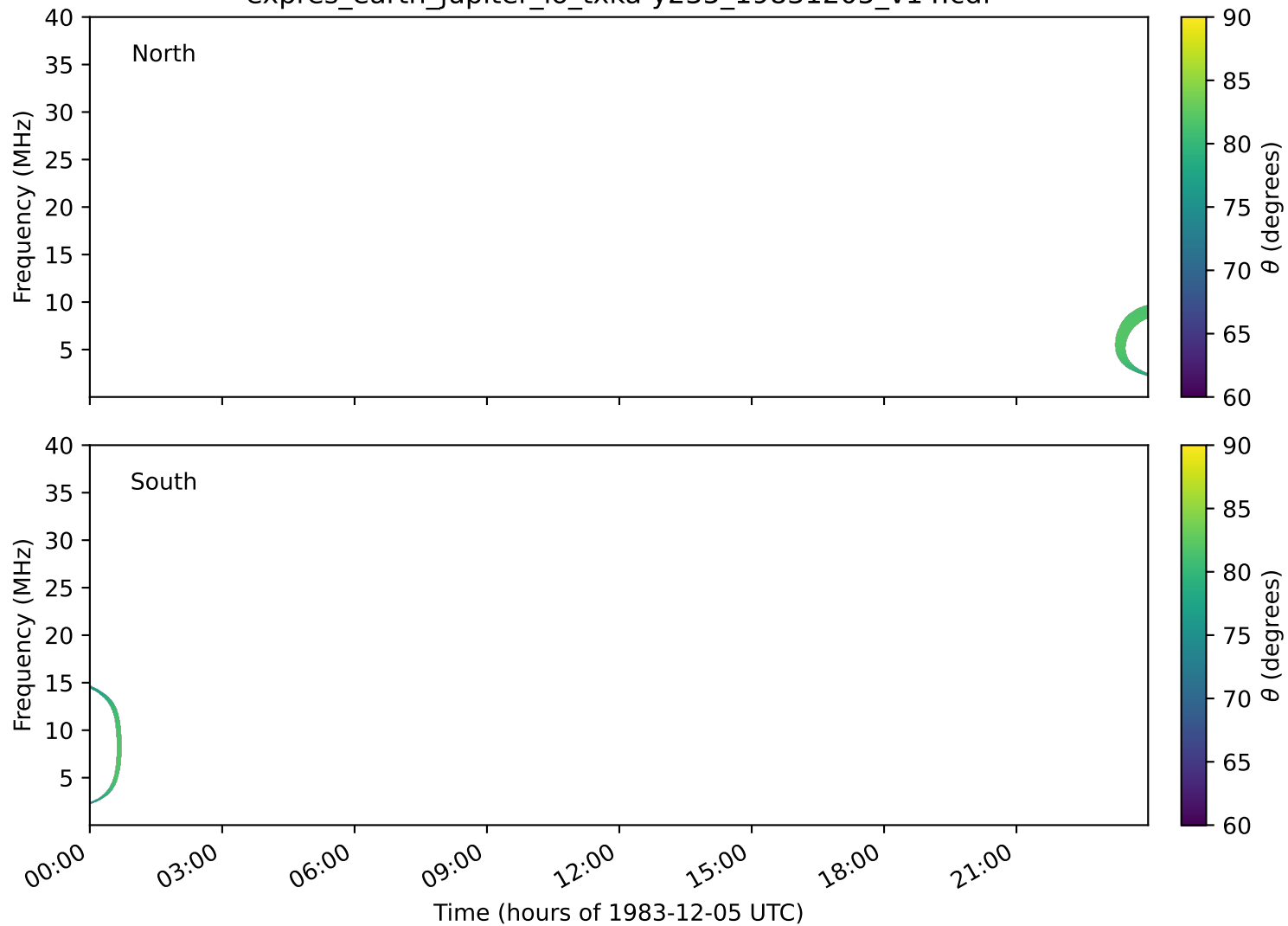
expres_earth_jupiter_io_txka-y235_19831205_v14.cdf
