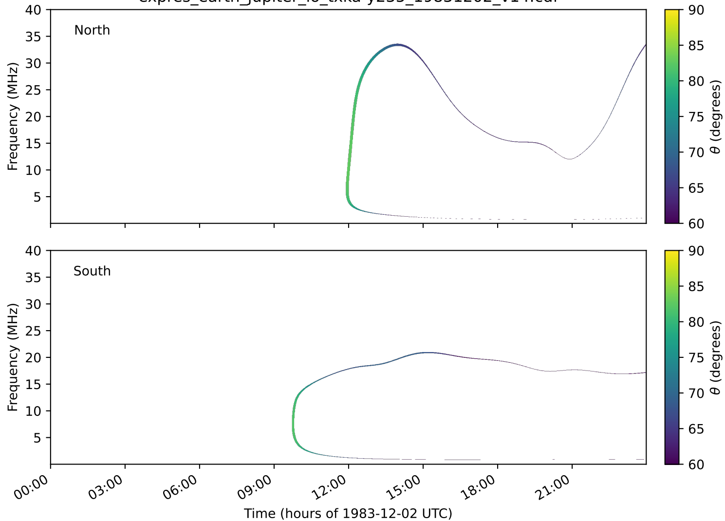
expres_earth_jupiter_io_txka-y235_19831202_v14.cdf
