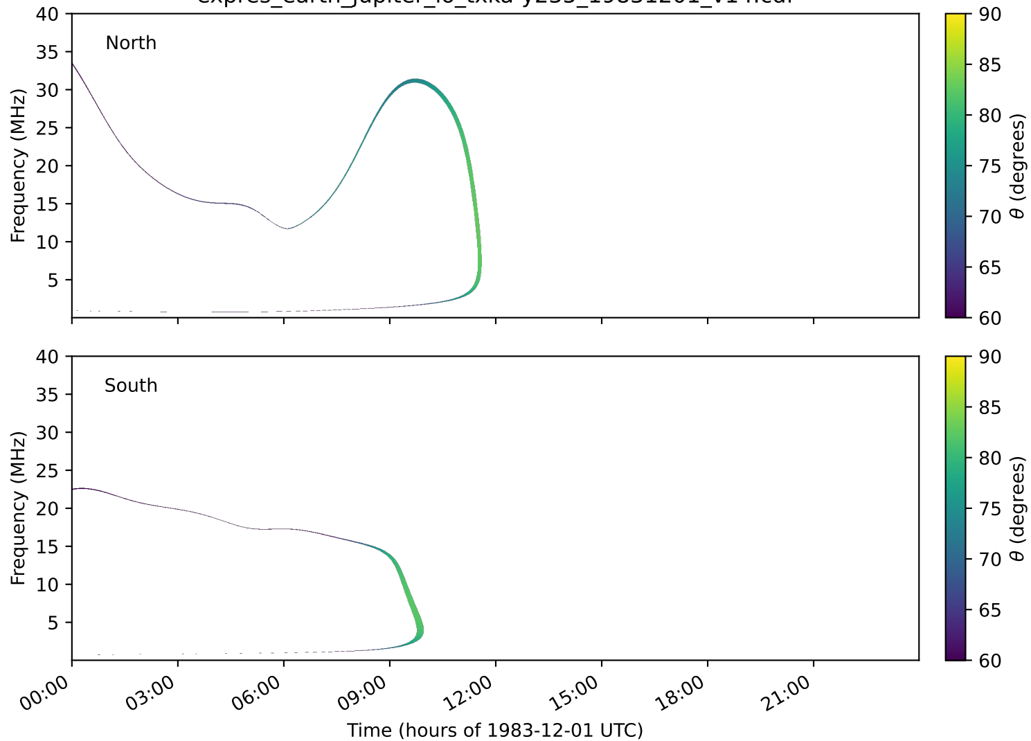
expres_earth_jupiter_io_txka-y235_19831201_v14.cdf
