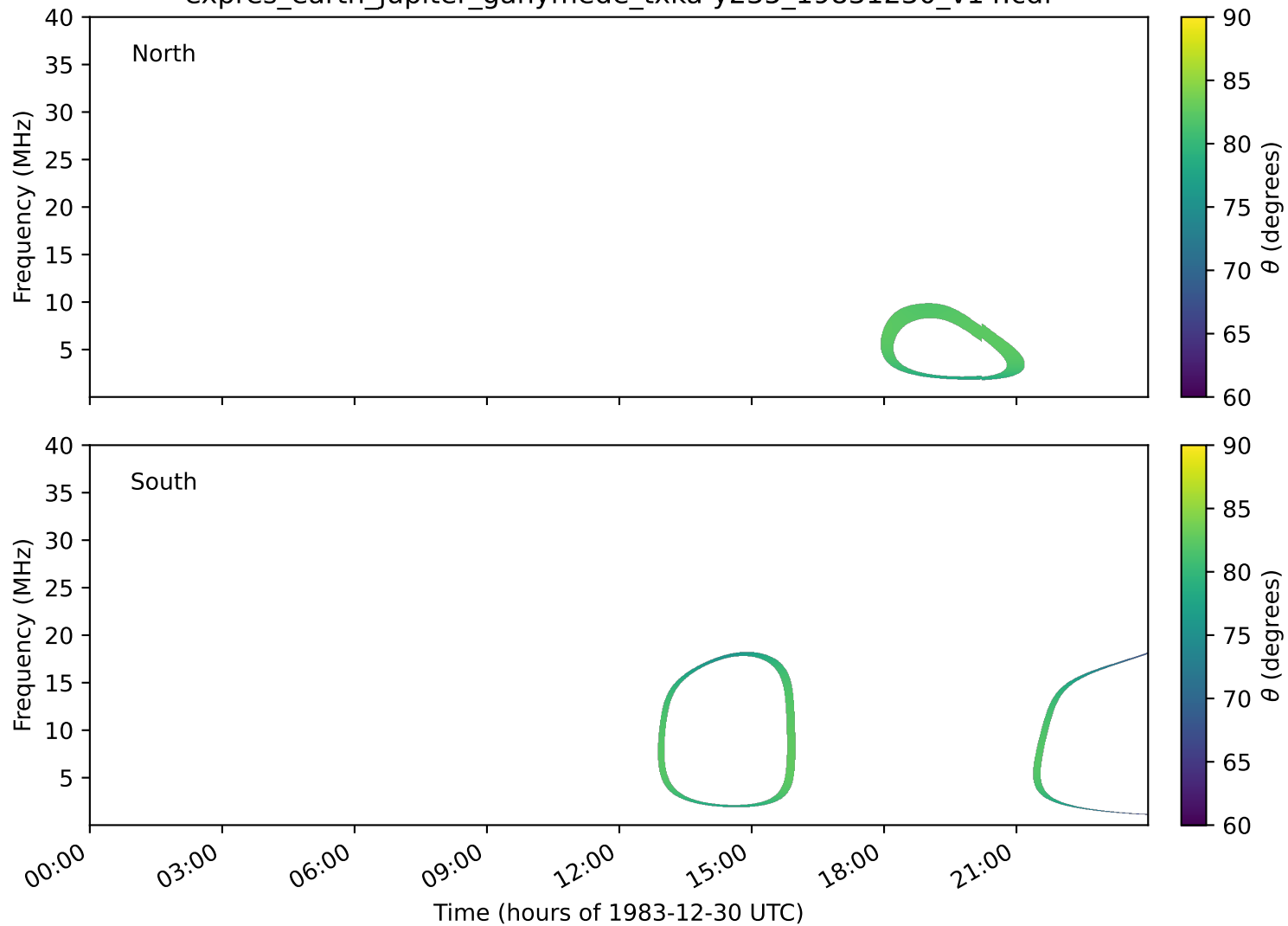
expres_earth_jupiter_ganymede_txka-y235_19831230_v14.cdf
