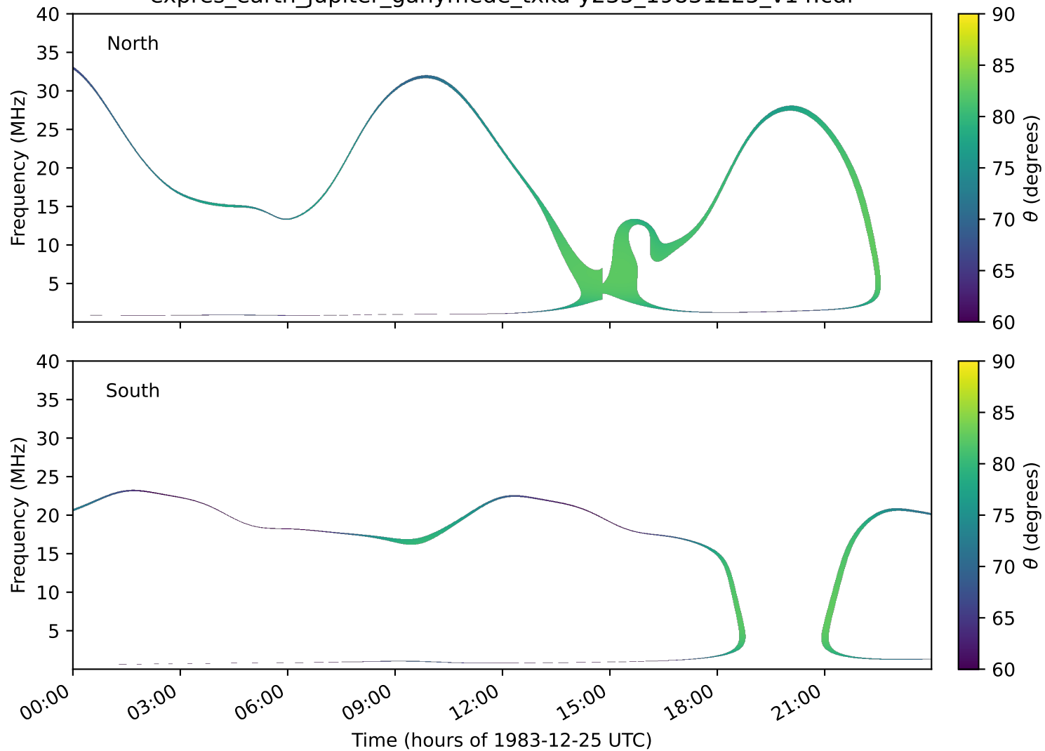
expres_earth_jupiter_ganymede_txka-y235_19831225_v14.cdf
