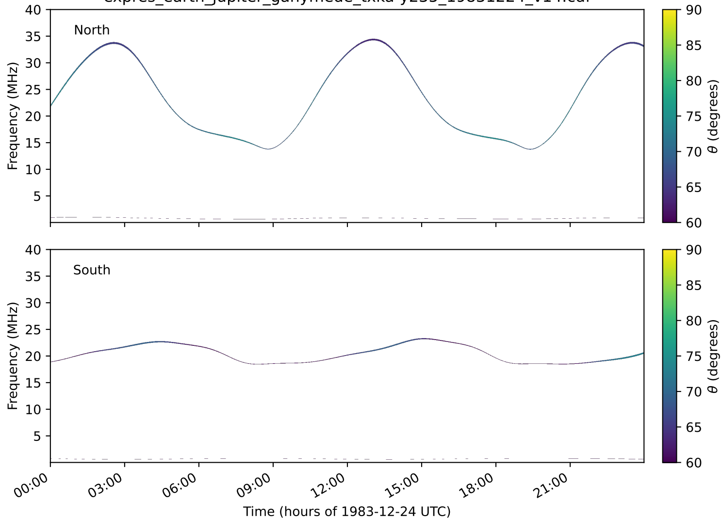
expres_earth_jupiter_ganymede_txka-y235_19831224_v14.cdf
