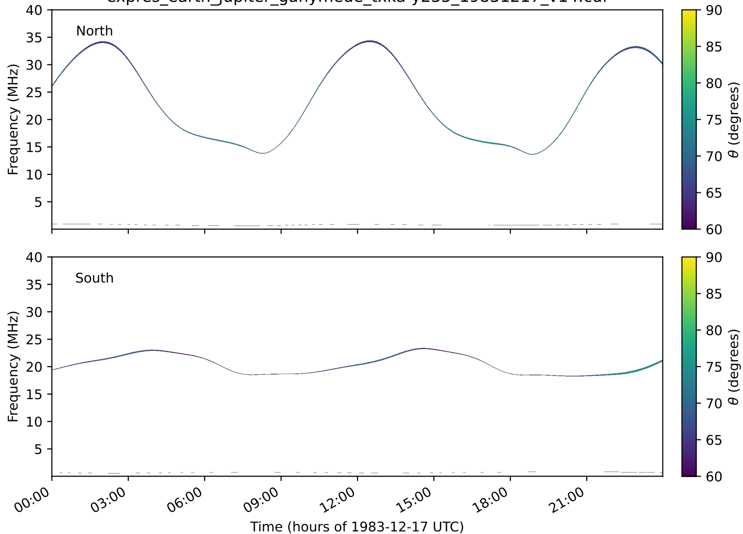
expres_earth_jupiter_ganymede_txka-y235_19831217_v14.cdf
