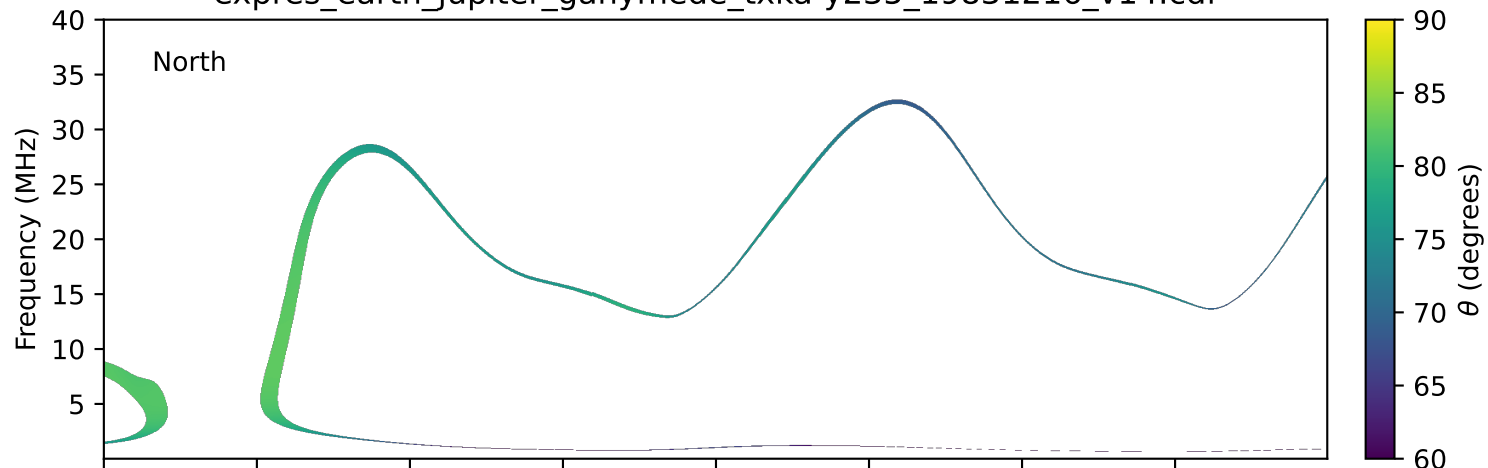
expres_earth_jupiter_ganymede_txka-y235_19831216_v14.cdf
