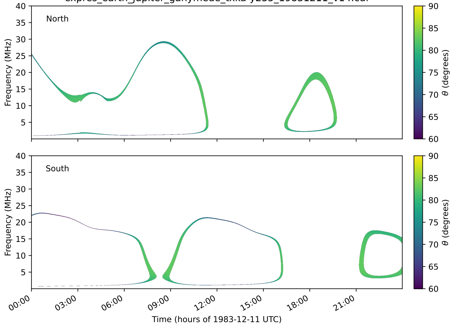
expres_earth_jupiter_ganymede_txka-y235_19831211_v14.cdf
