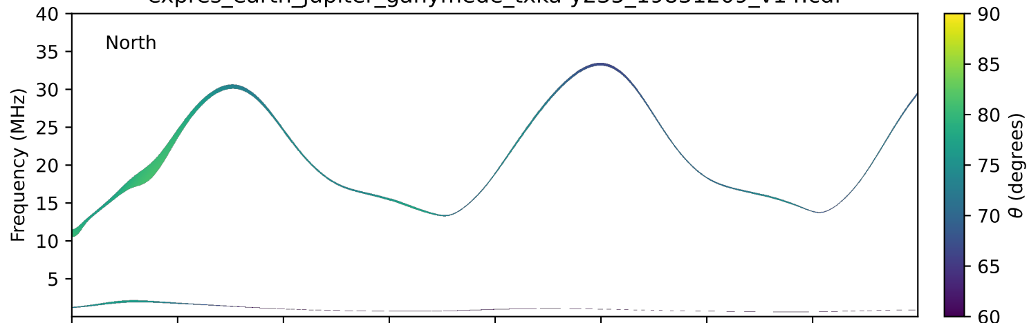
expres_earth_jupiter_ganymede_txka-y235_19831209_v14.cdf
