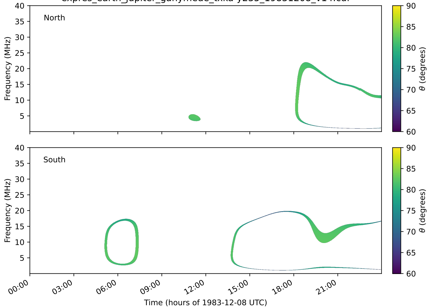
expres_earth_jupiter_ganymede_txka-y235_19831208_v14.cdf
