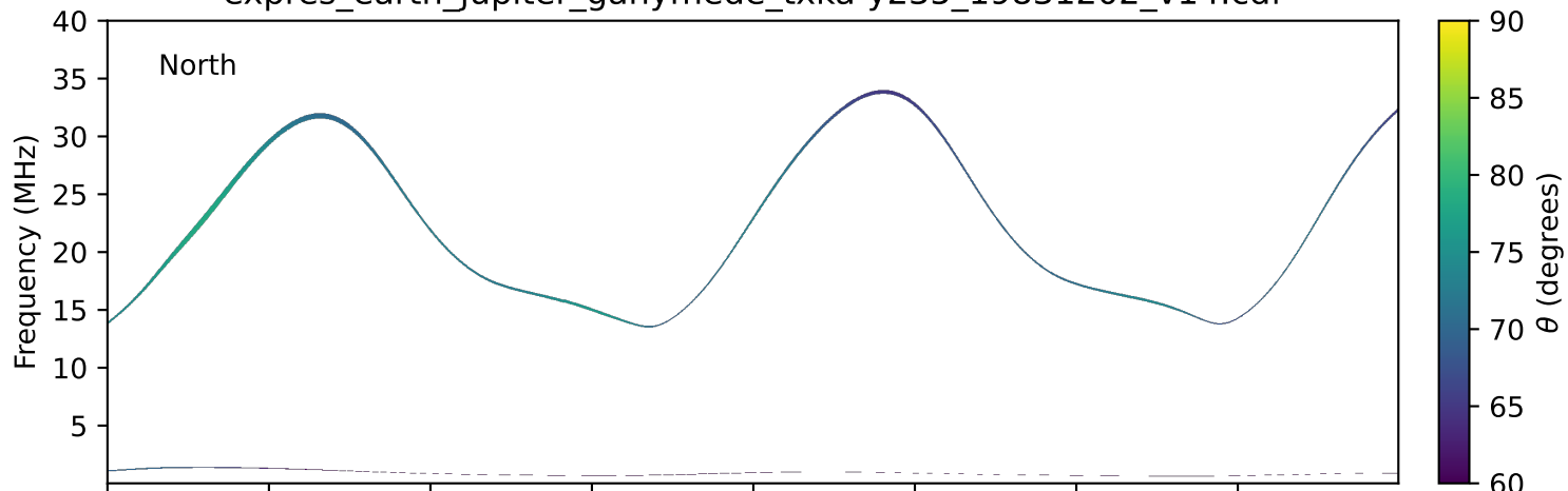
expres_earth_jupiter_ganymede_txka-y235_19831202_v14.cdf
