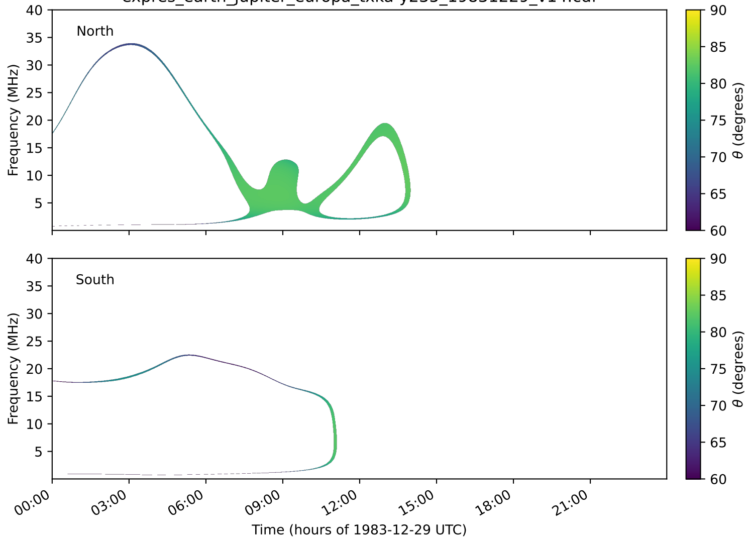
expres_earth_jupiter_europa_txka-y235_19831229_v14.cdf
