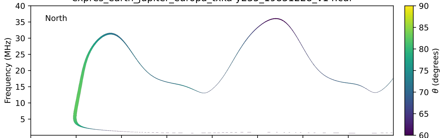
expres_earth_jupiter_europa_txka-y235_19831228_v14.cdf
