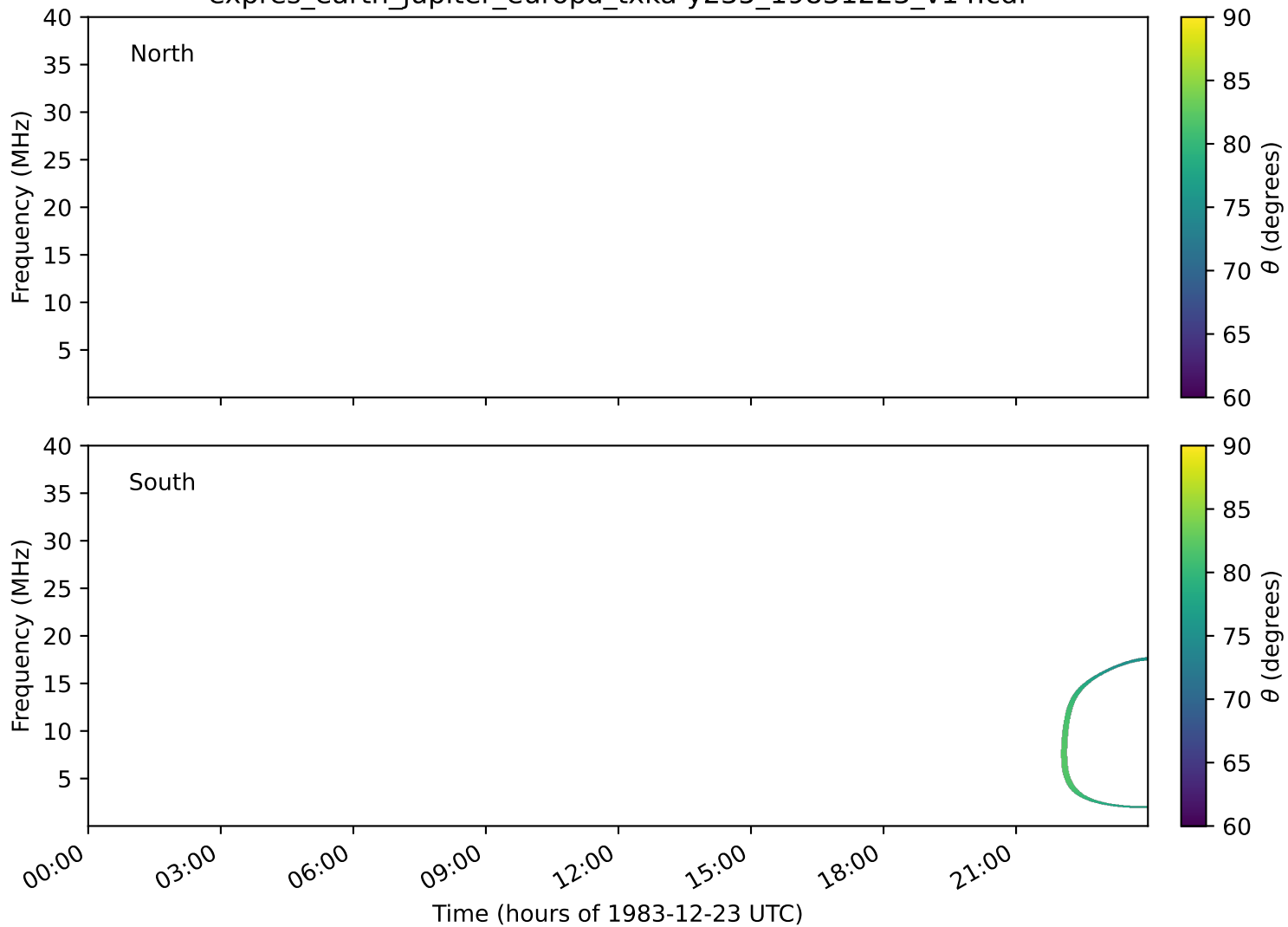
expres_earth_jupiter_europa_txka-y235_19831223_v14.cdf
