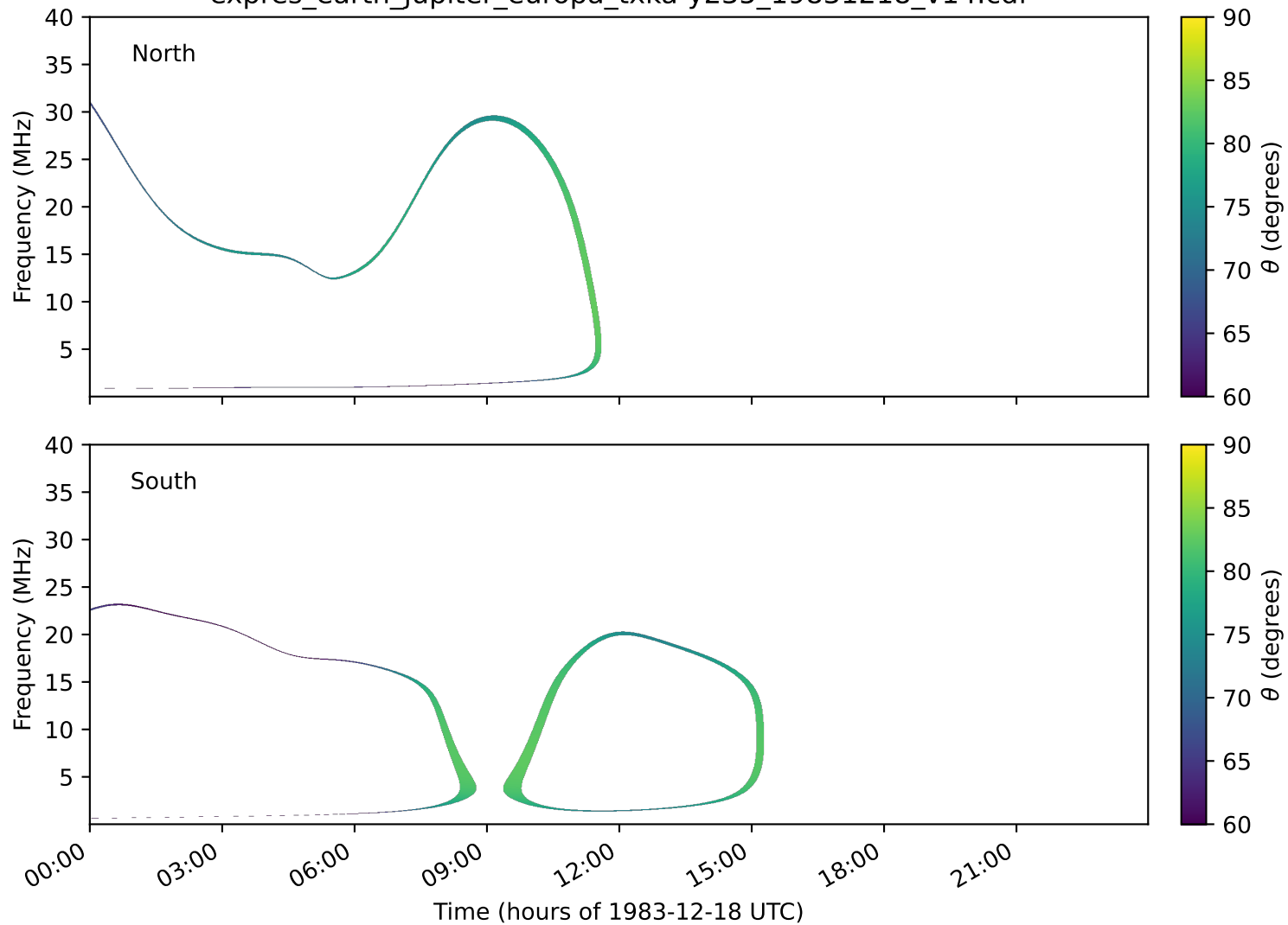
expres_earth_jupiter_europa_txka-y235_19831218_v14.cdf
