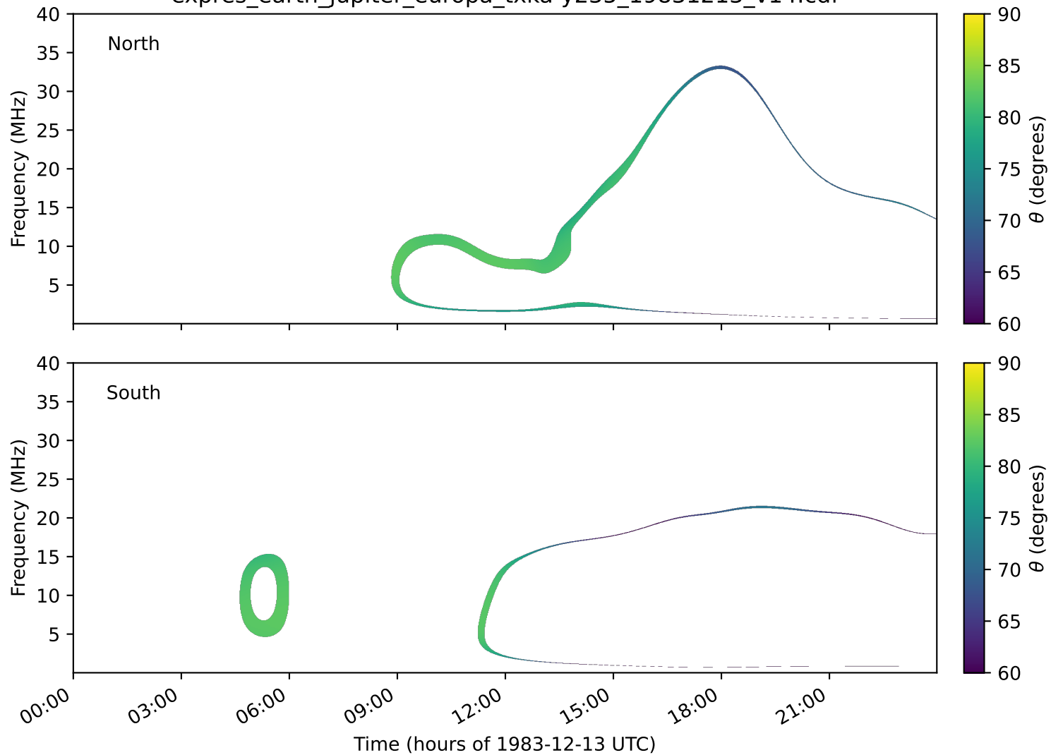
expres_earth_jupiter_europa_txka-y235_19831213_v14.cdf
