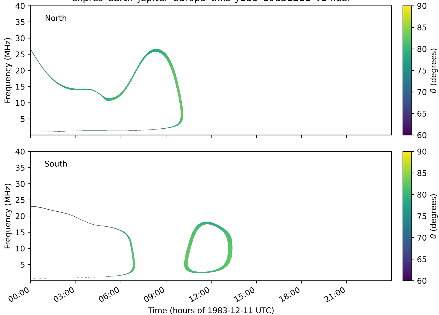
expres_earth_jupiter_europa_txka-y235_19831211_v14.cdf
