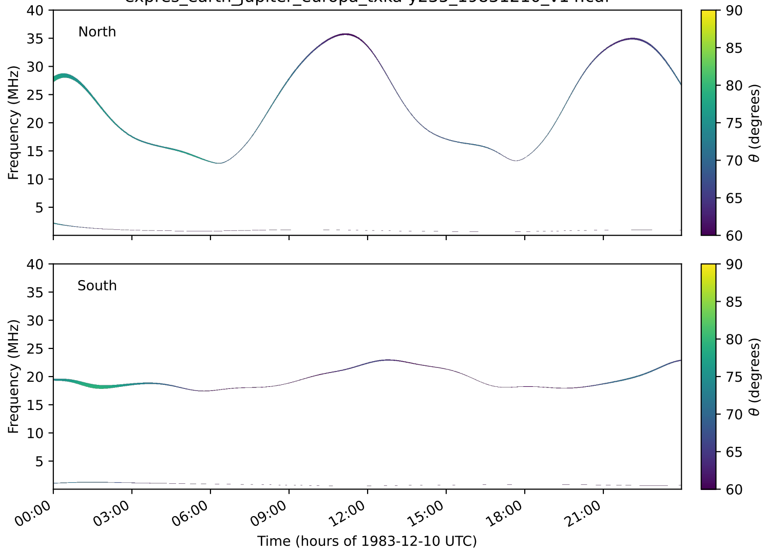
expres_earth_jupiter_europa_txka-y235_19831210_v14.cdf
