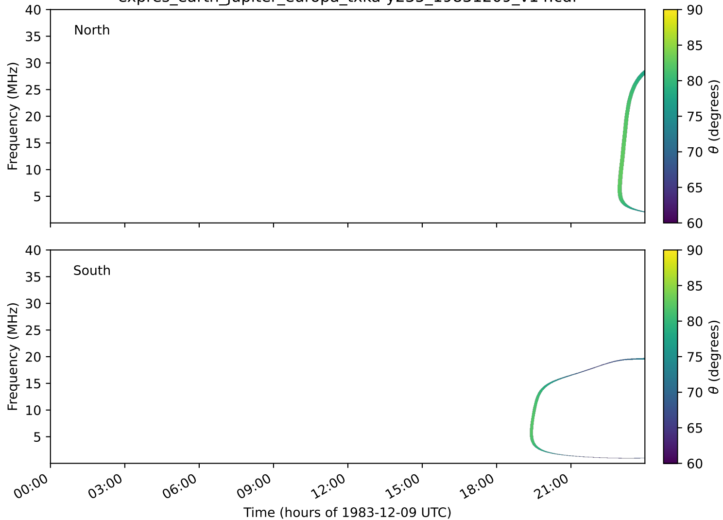
expres_earth_jupiter_europa_txka-y235_19831209_v14.cdf
