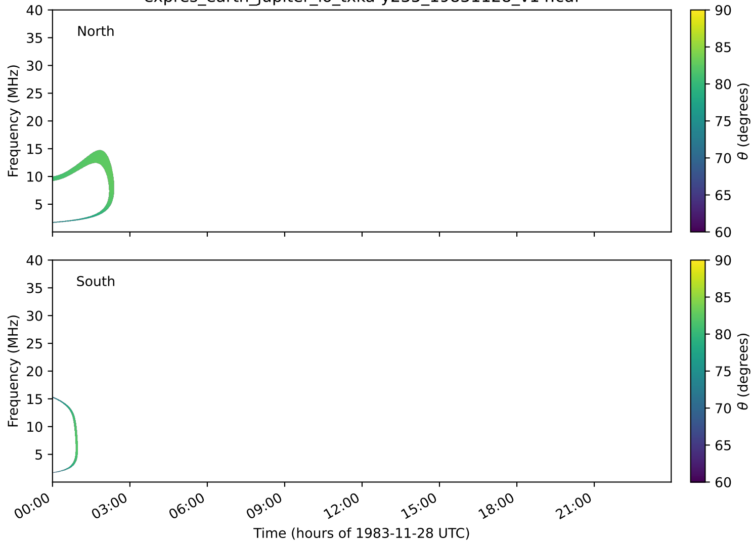
expres_earth_jupiter_io_txka-y235_19831128_v14.cdf
