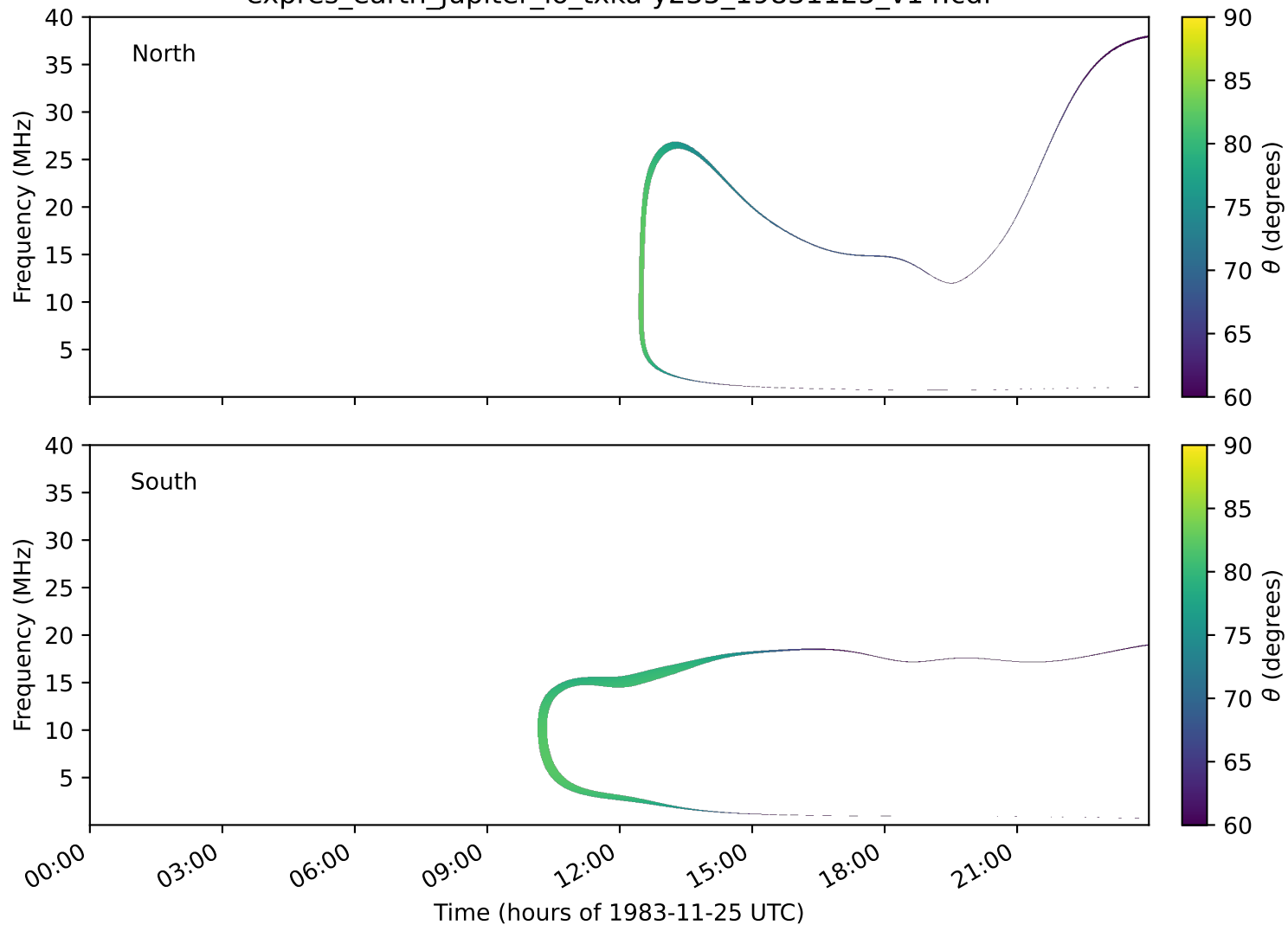
expres_earth_jupiter_io_txka-y235_19831125_v14.cdf
