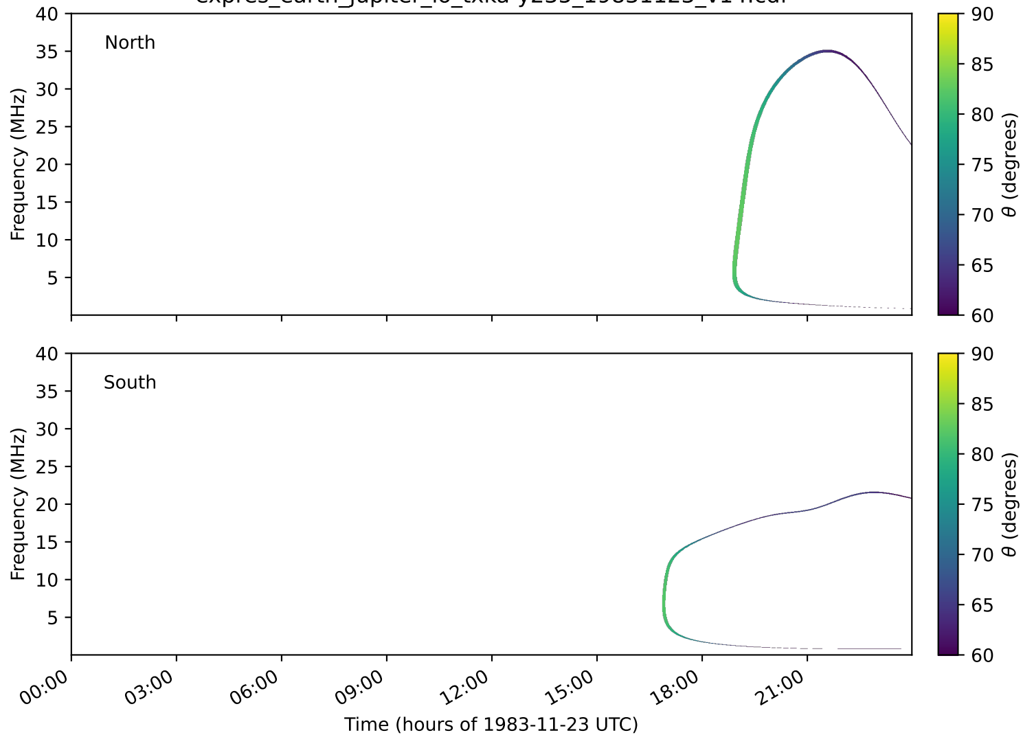
expres_earth_jupiter_io_txka-y235_19831123_v14.cdf
