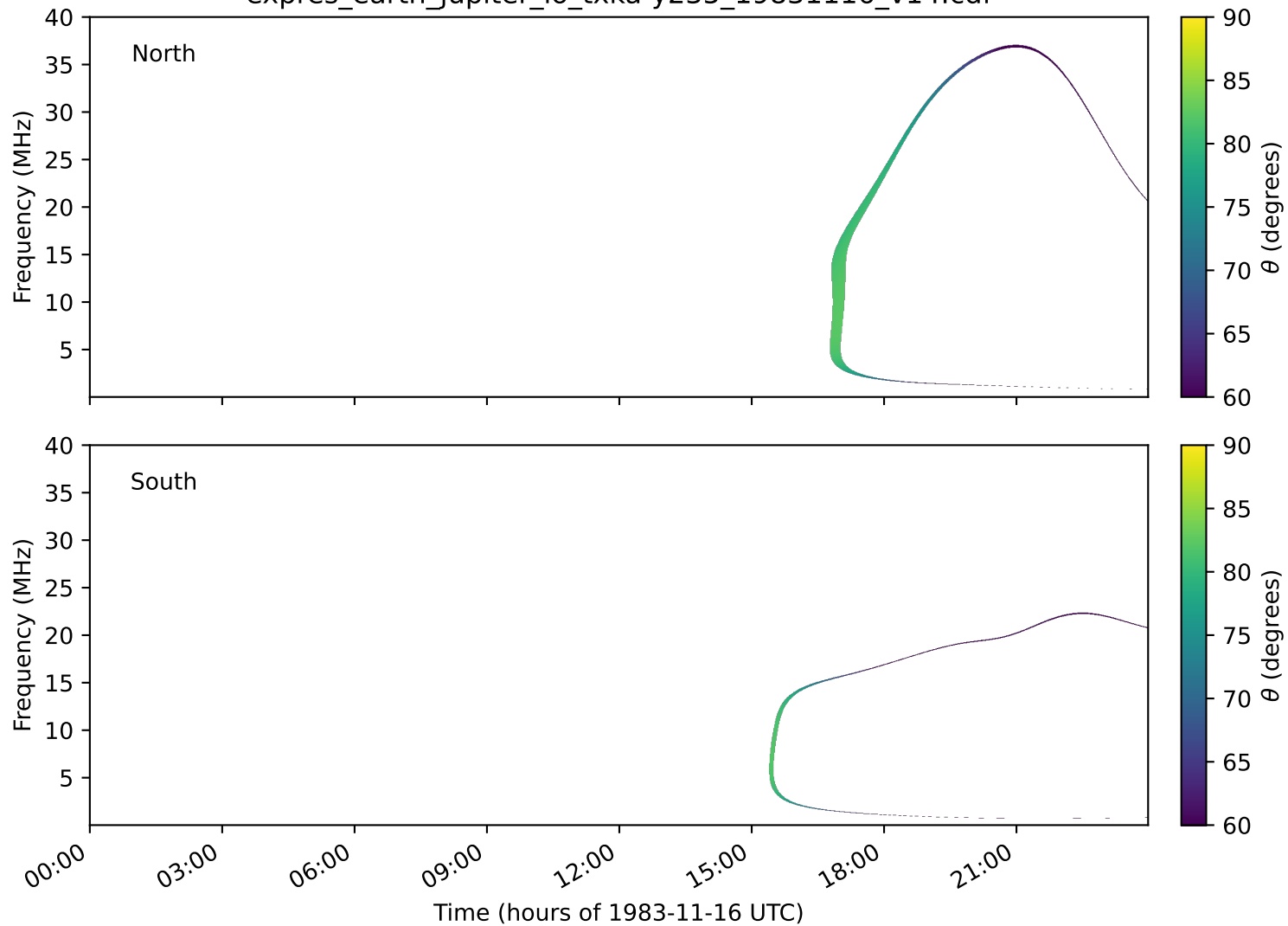
expres_earth_jupiter_io_txka-y235_19831116_v14.cdf
