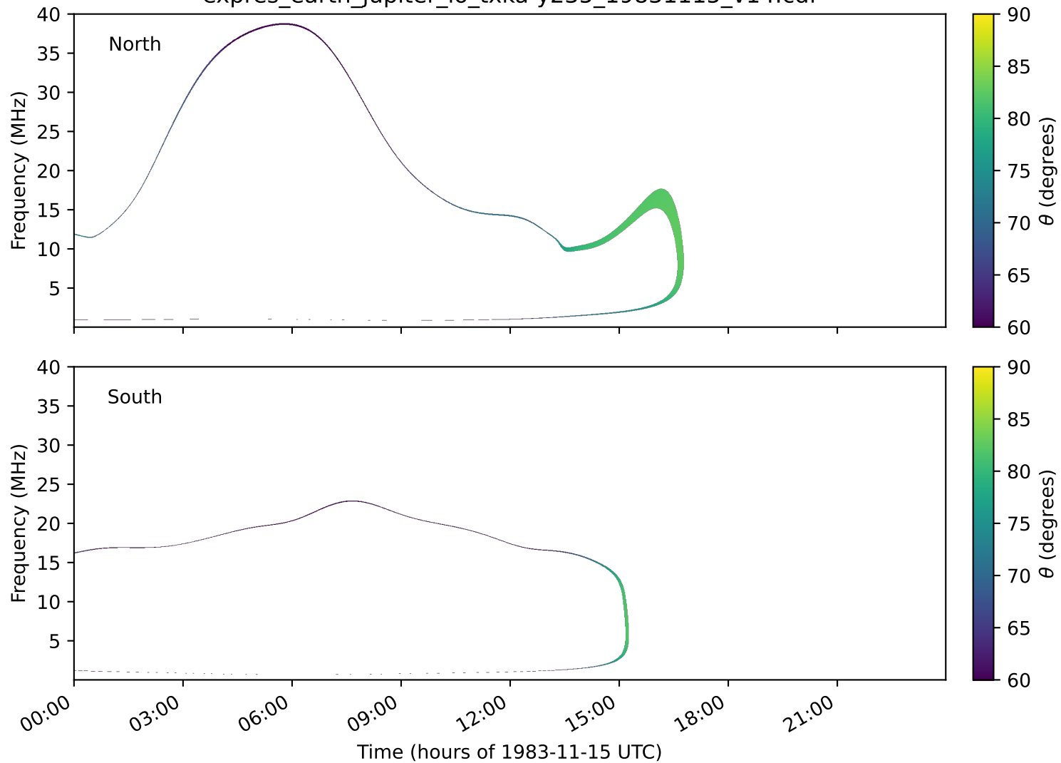
expres_earth_jupiter_io_txka-y235_19831115_v14.cdf
