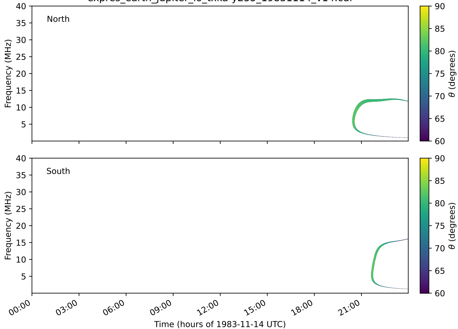
expres_earth_jupiter_io_txka-y235_19831114_v14.cdf
