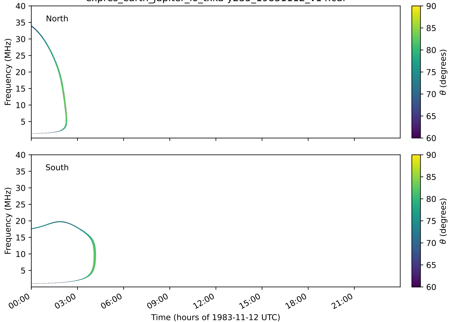
expres_earth_jupiter_io_txka-y235_19831112_v14.cdf
